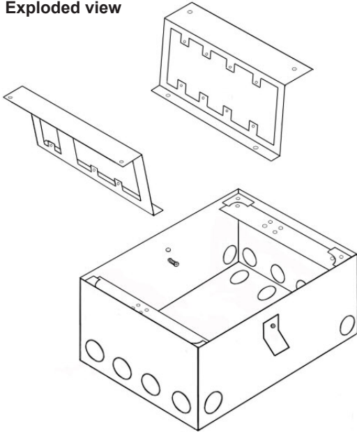
Exploded view
